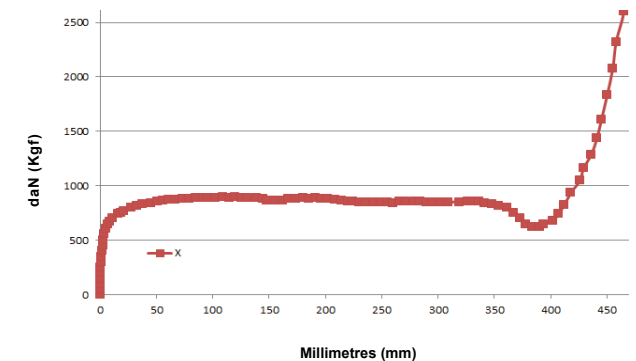
Maximum tension in the lifeline with the X-60 absorber
