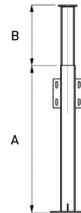
Model P-10/T Telescopic steel | Stainless steel post
