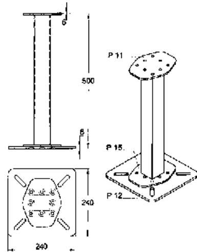
P-10 Floor mounted stainless steel post
