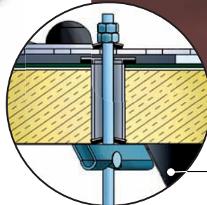
Detail of overlaying mounting with compression tube and rocker arm bolt
